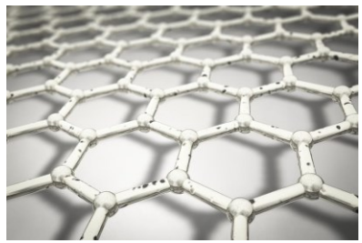
Nanomaterials
