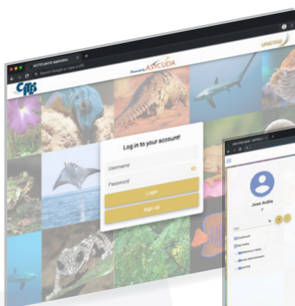
Login screen
