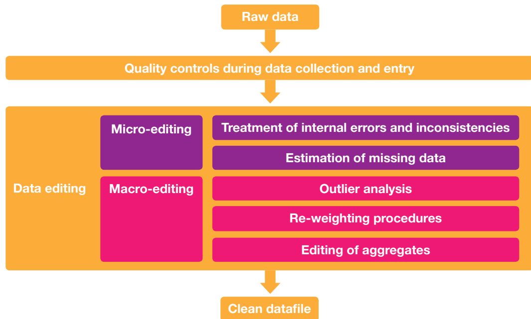
Figure 7 Steps in data validation
