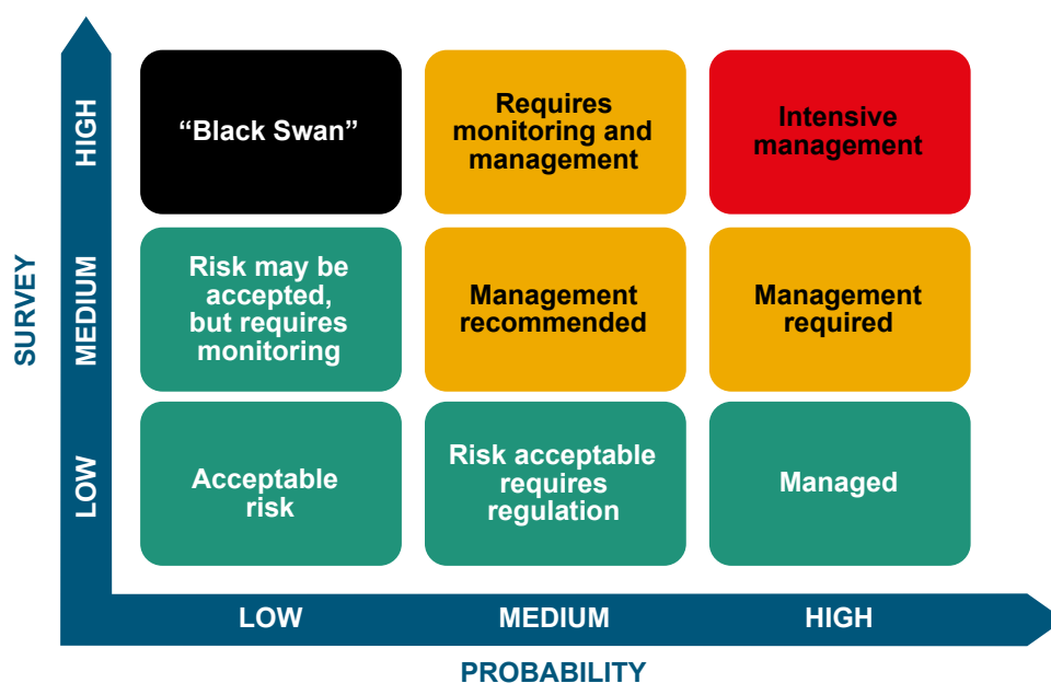
Figure 16: Quantifying risks
