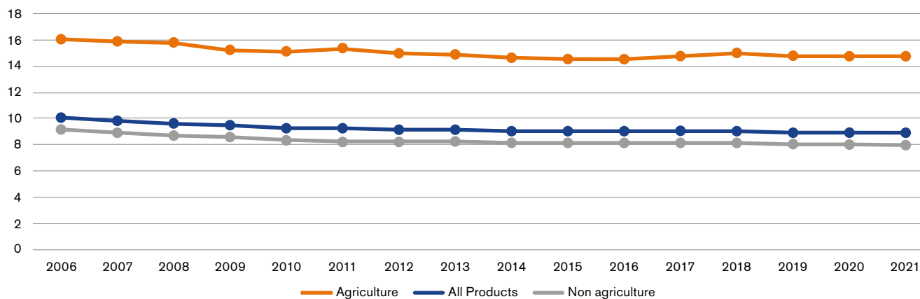
Figure 1. Applied MFN average tariffs (simple average in per cent)
