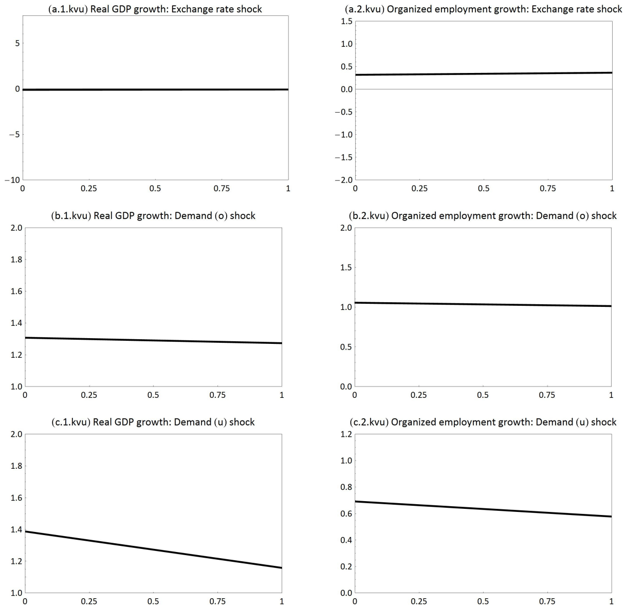
Figure 5: Sensitivity analysis on Kaldor-Verdoorn coefficient for the unorganized sectors (it includes agriculture).
